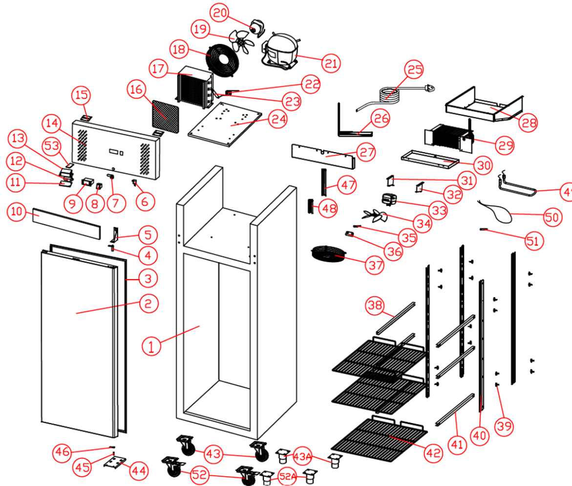
EXPLODED DIAGRAM XURF400SFV
